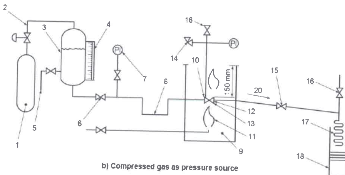
Figure 1. Typical Fire-Test System Using Compressed Gas as the Pressure Source
